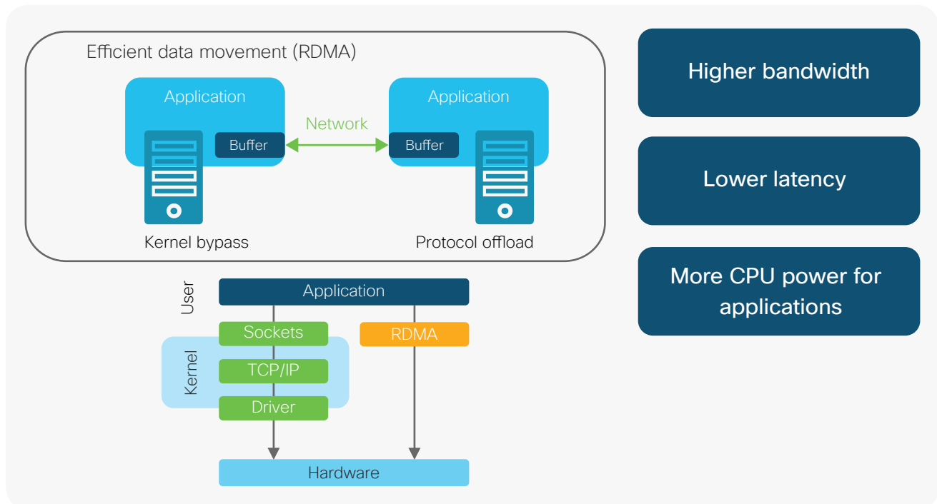
Figure 1. Remove Data Memory Access (RDMA)
